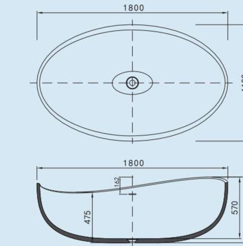
GM-8015 Freestanding Bathtub Size : 1800x1100x620mm Material : Solid Surface
