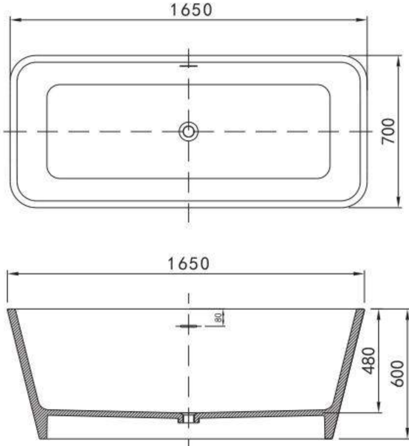
GM-8020 Freestanding Bathtub Size : 1650x700x600mm Material : Solid Surface
