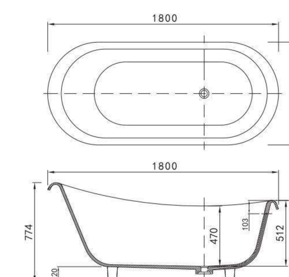
GM-8002 Freestanding Bathtub Size : 1800x800x774mm Material : Solid Surface
