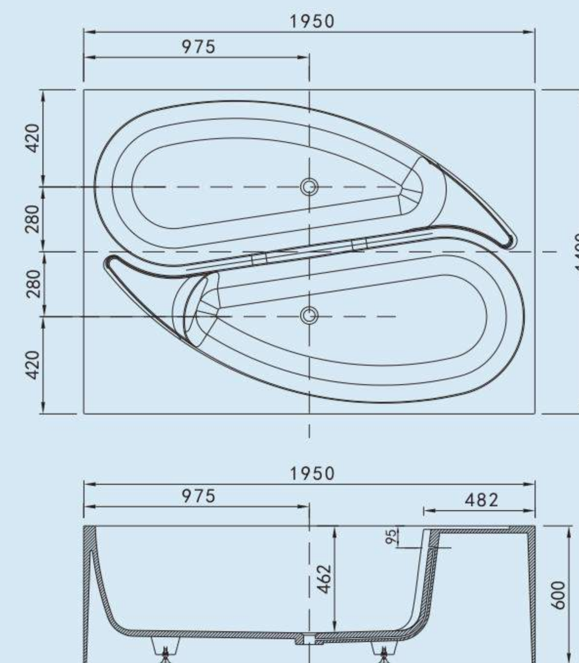
GM-8003 Freestanding Bathtub Size : 1950x1400x600mm Material : Solid Surface
