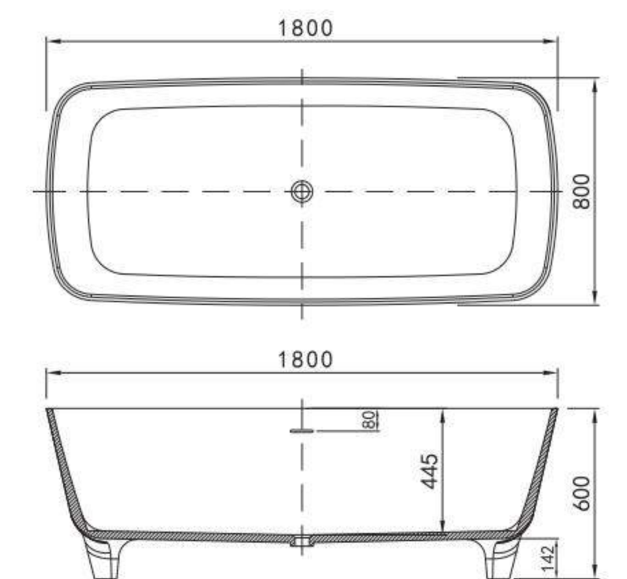
GM-8005 Freestanding Bathtub Size : 1800x800x600mm Material : Solid Surface
