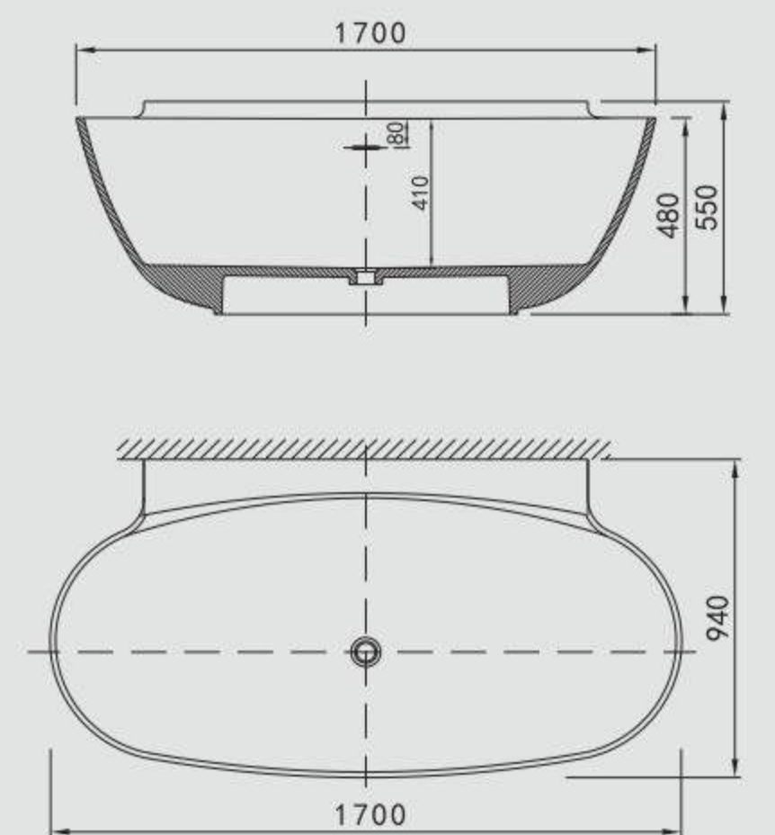
GM-8007 Freestanding Bathtub Size : 1700x940x550mm Material : Solid Surface
