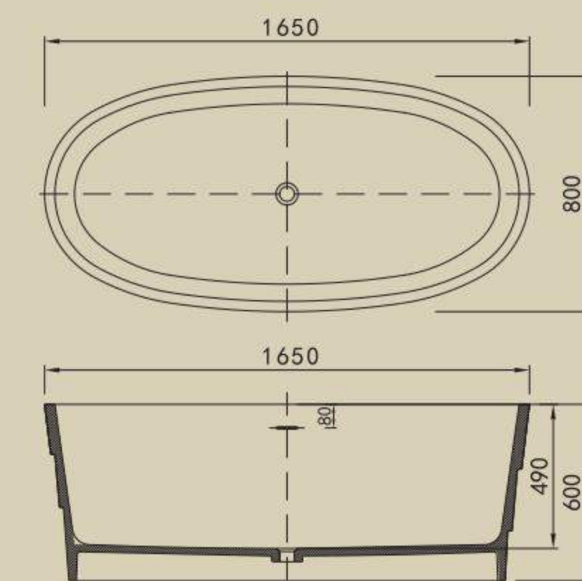
GM-8022 Freestanding Bathtub Size : 1650x800x600mm Material : Solid Surface with golden gel coat
