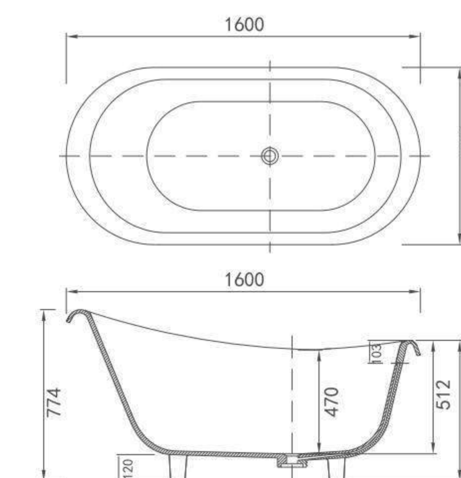
GM-8002S Freestanding Bathtub Size : 1600x800x774mm Material : Solid Surface
