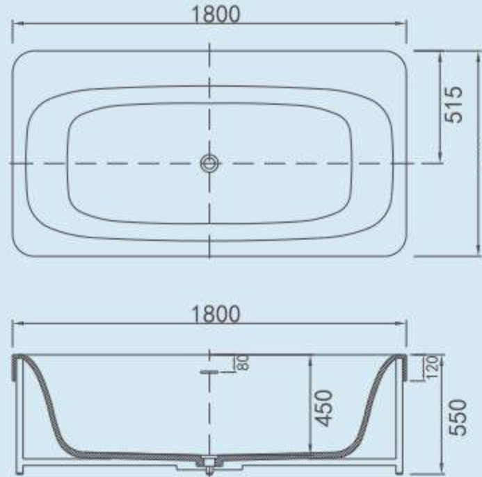
GM-8011 Freestanding Bathtub Size : 1800x940x550mm Material : Solid Surface
