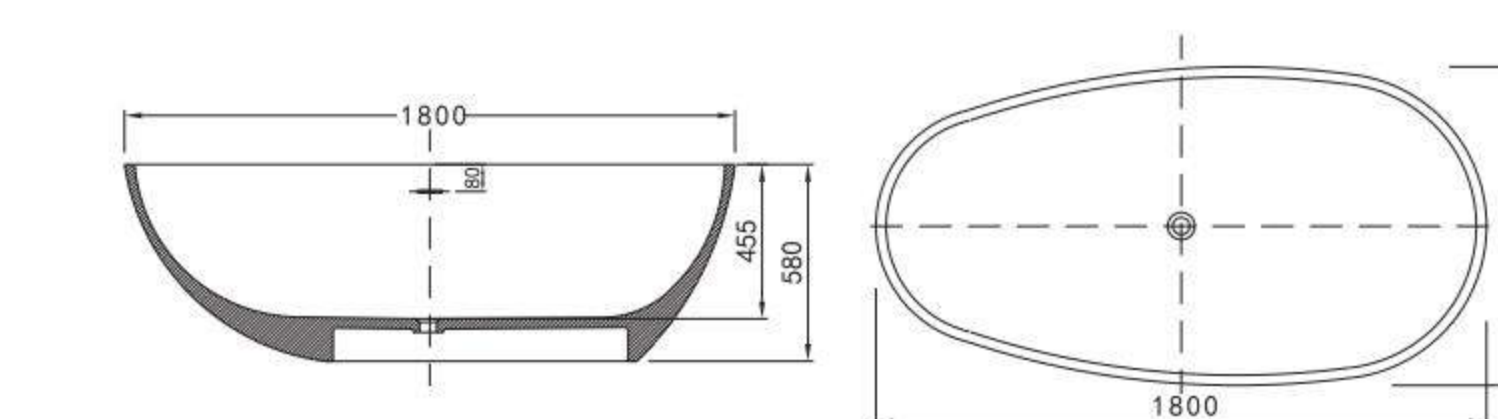
GM-8004 Freestanding Bathtub Size : 1800x900x580mm Material : Solid Surface
