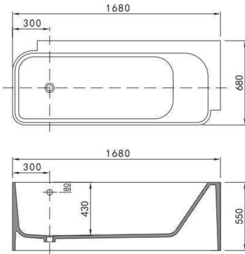
GM-8018 Freestanding Bathtub Size : 1680x680x550mm Material : Solid Surface
