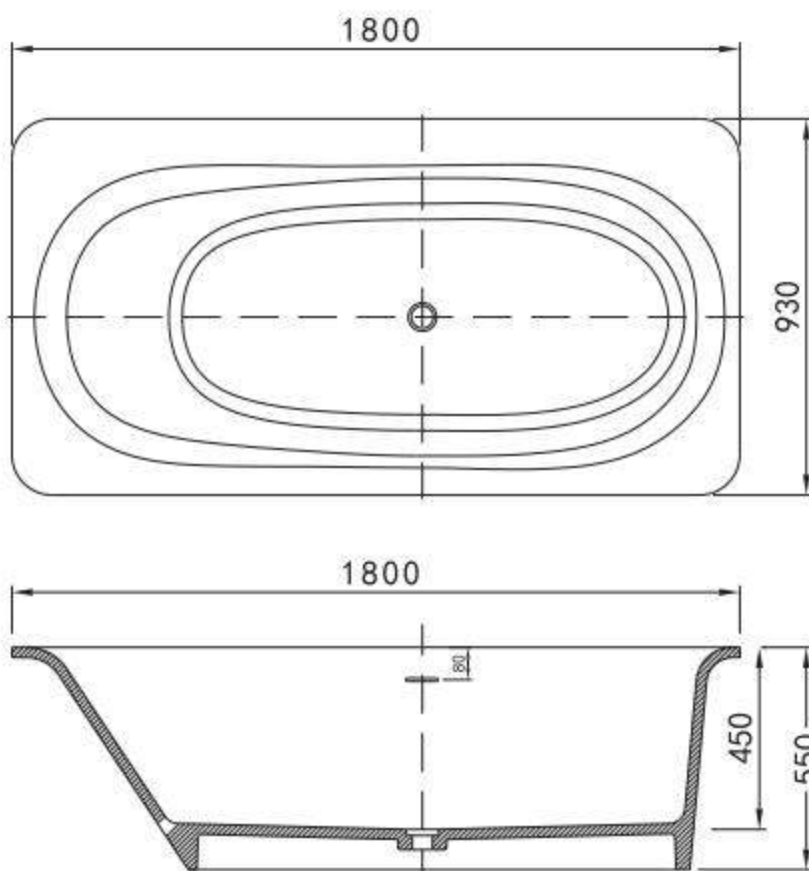
GM-8012 Freestanding Bathtub Size : 1800x930x550mm Material : Solid Surface
