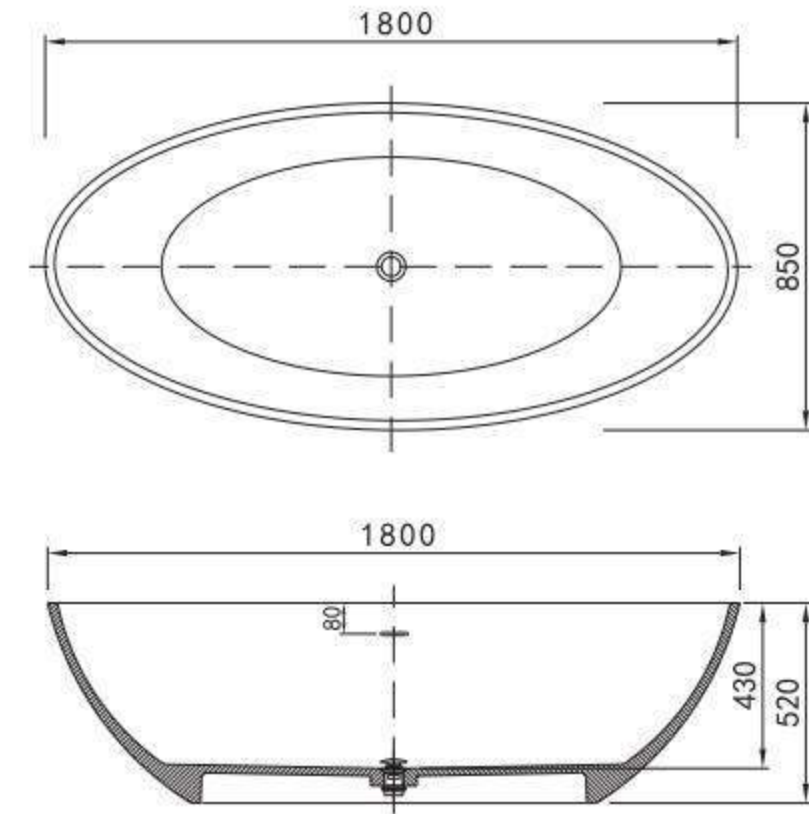
GM-8014 Freestanding Bathtub Size : 1800x850x520mm Material : Solid Surface
